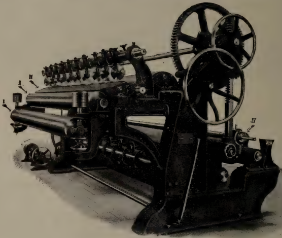
REAR VIEW SHOWING SLITTERS.
